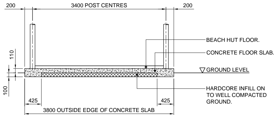
SECTION THRO' BASE
